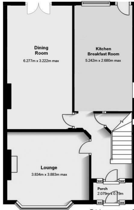
Ground Floor Approx. 48.8 sq. metres (524.8 sq. feet)
